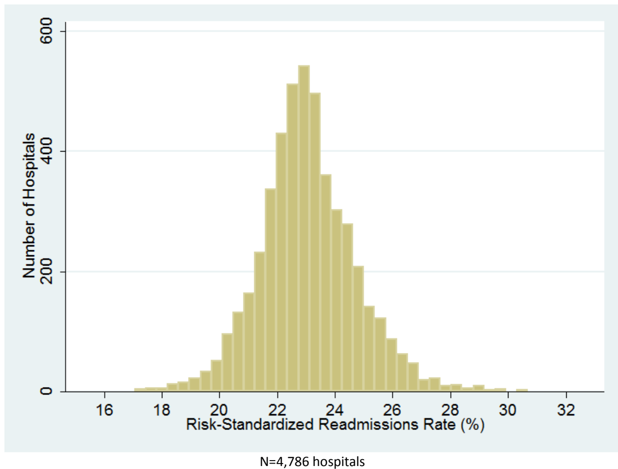
Figure 4 – Distribution of Hospital 30-Day HF RSRRs between July 2009 and June 2012
